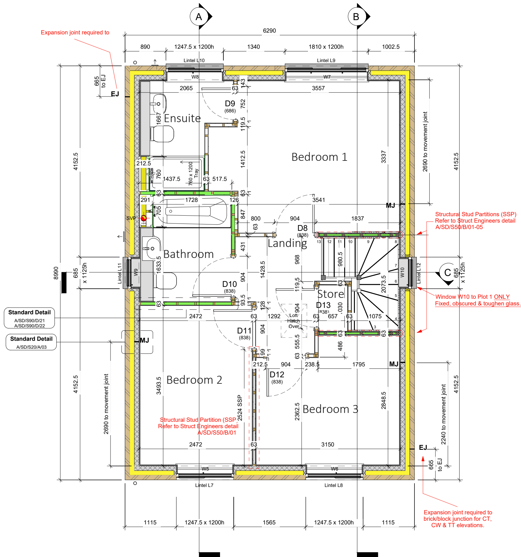
1 First Floor 1 : 50
